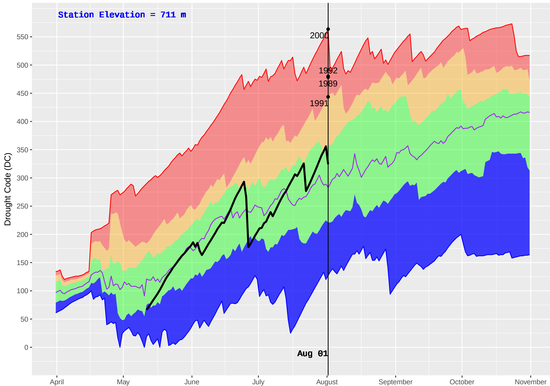
TOAD RIVER (126) : Historical (1981–2016) and Current (2018) Daily Drought Code (DC)
