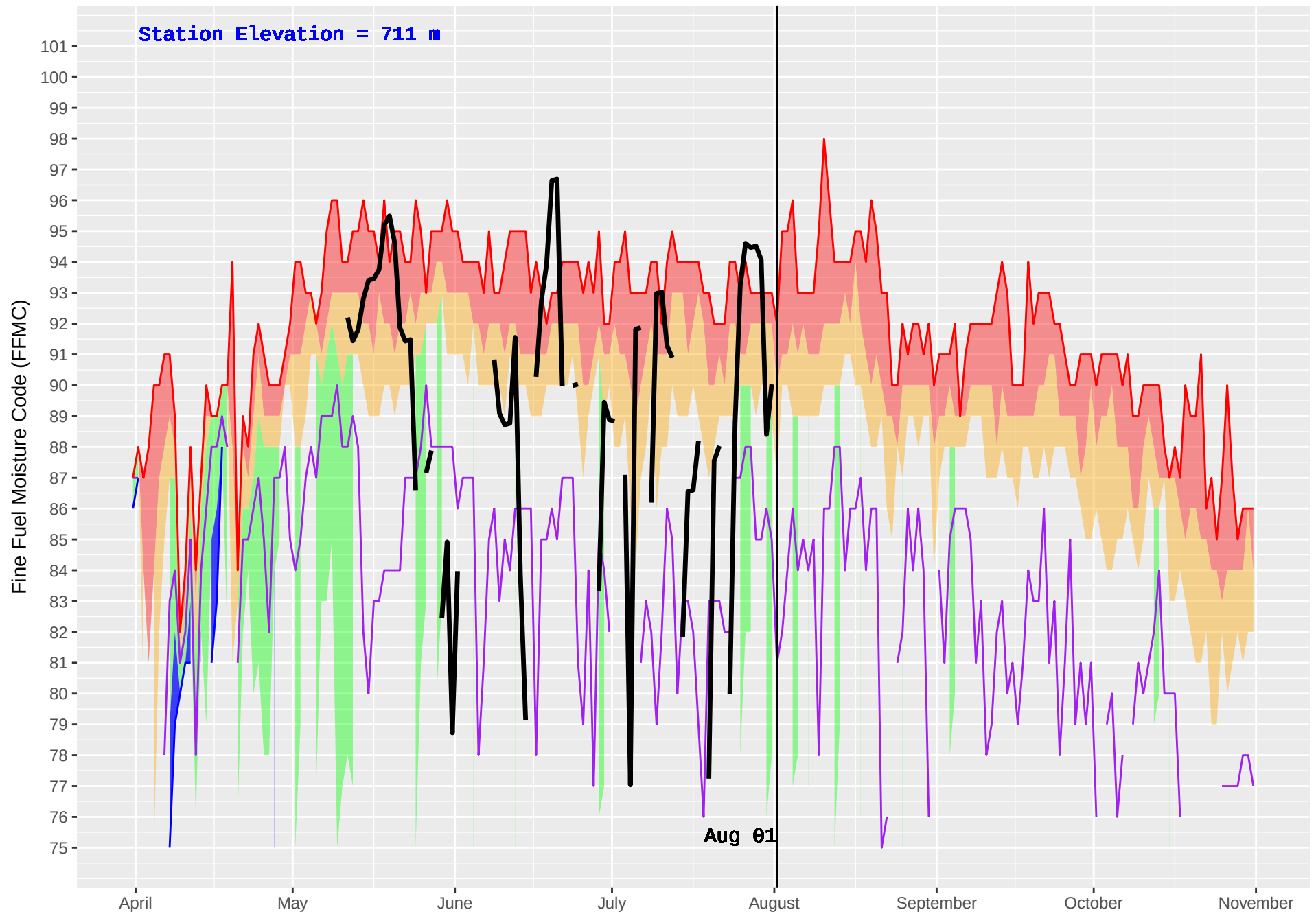
TOAD RIVER (126) : Historical (1981–2016) and Current (2018) Daily Fine Fuel Moisture Code (FFMC)
