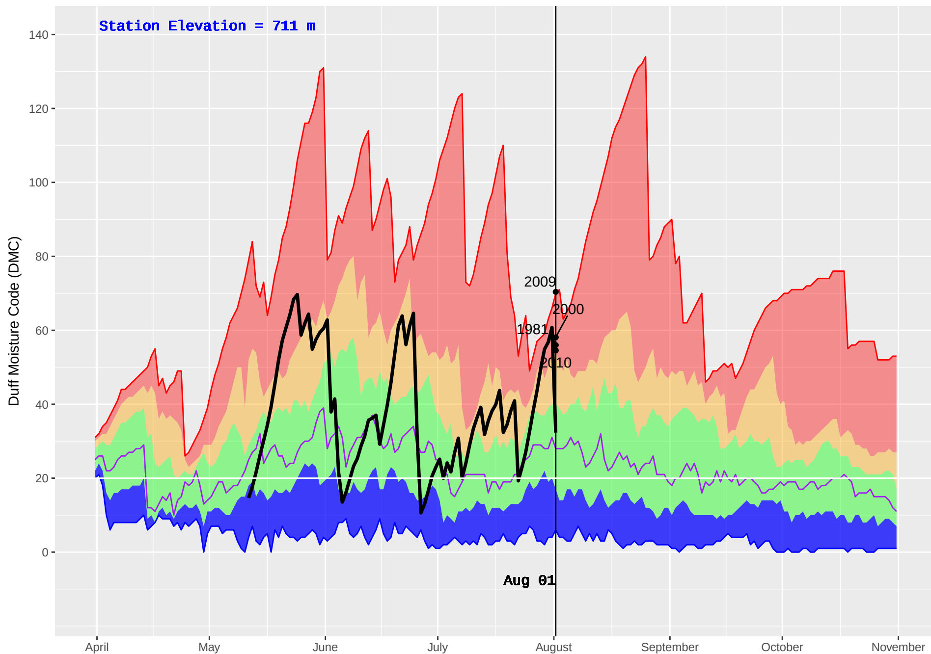
TOAD RIVER (126) : Historical (1981–2016) and Current (2018) Daily Duff Moisture Code (DMC)
